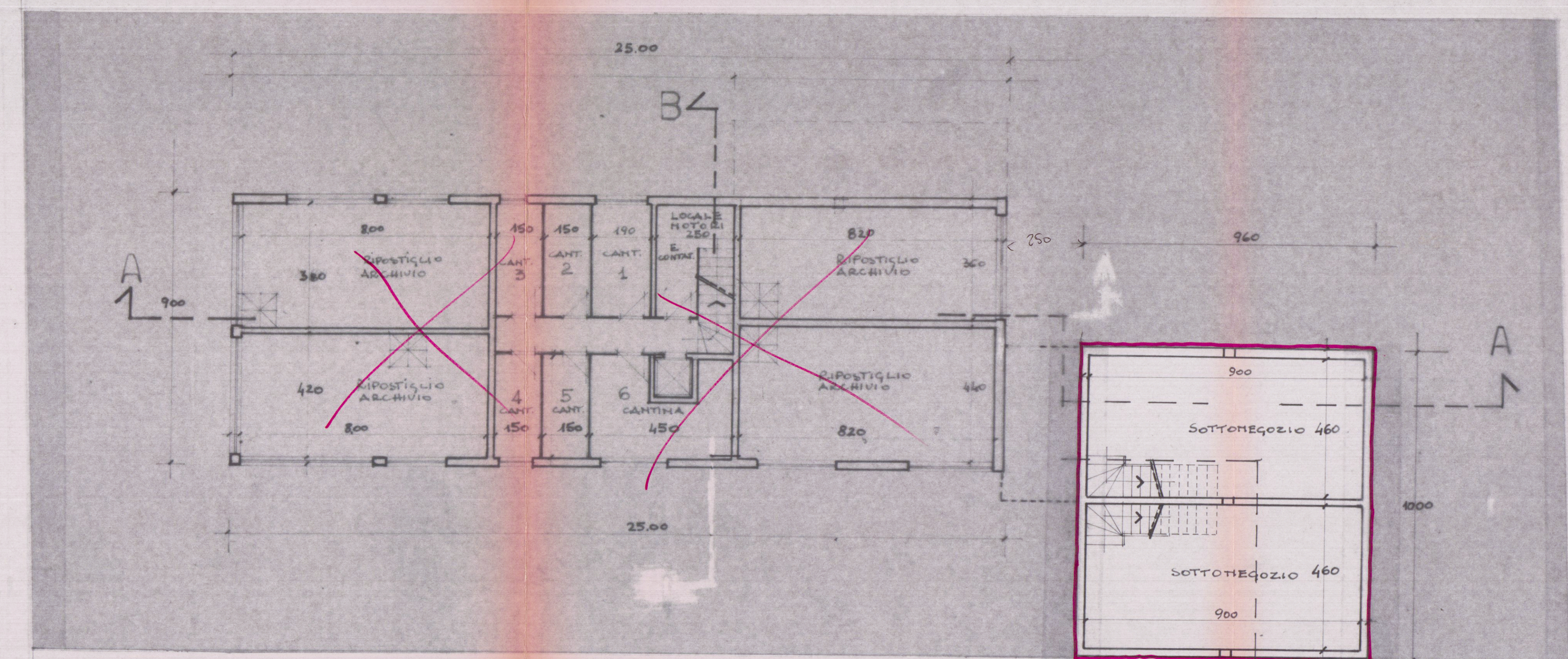
PIANO SEMINTERRATO RAPP. 1:100
